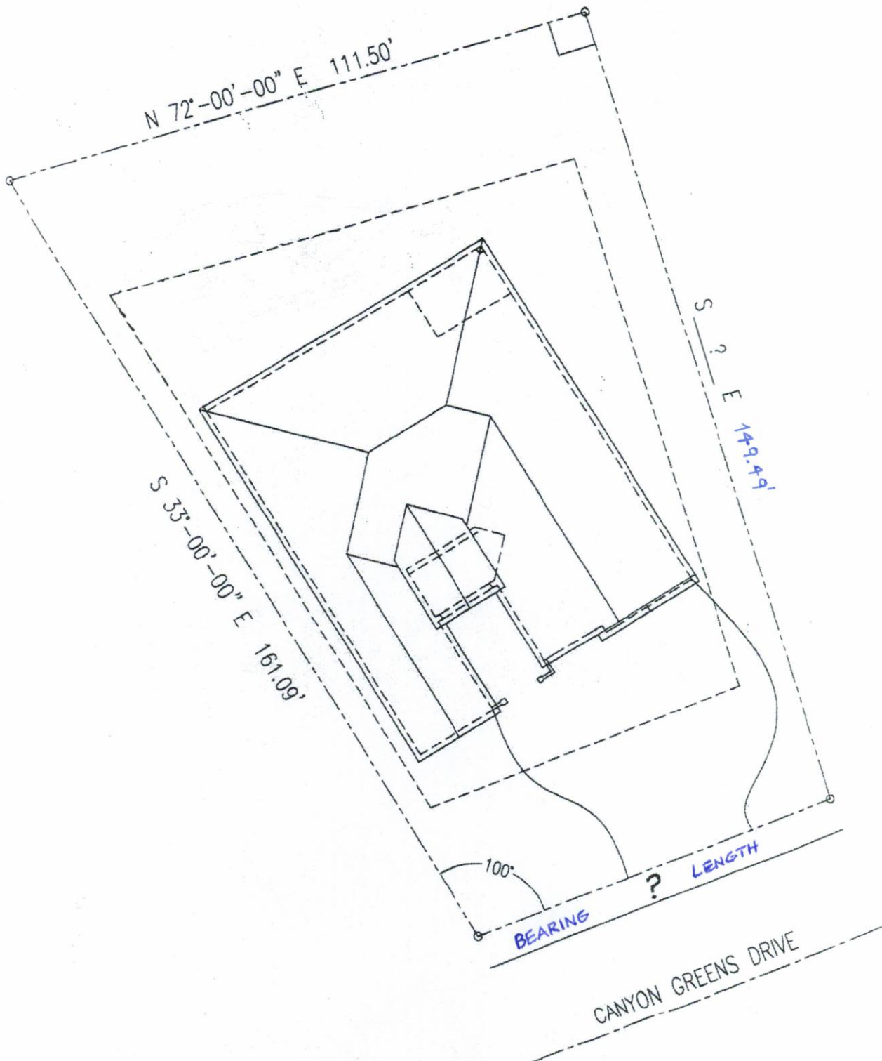
PLOT PLAN
